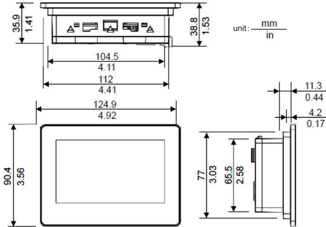
Figure 1-2 Dimensions for Touch Display
