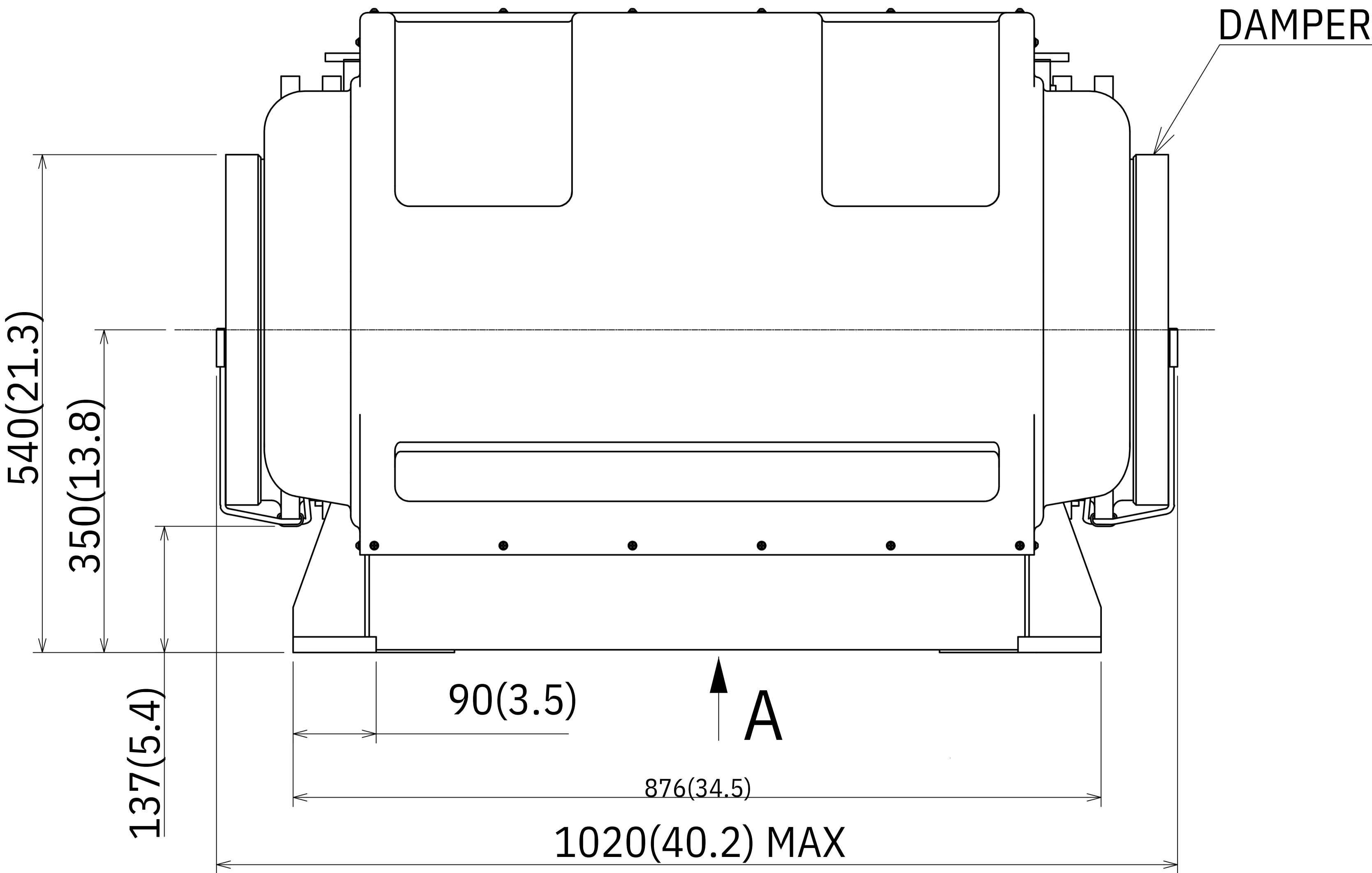
VIEW A
